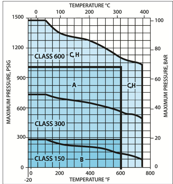
Figure 2. Trim Chart For Carbon Steel Body (ASTM A216, WCB)
